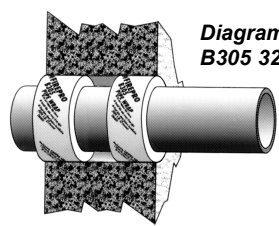
Diagram B - WALL SEALS All sizes B306 and B305-65 & larger sizes B305 use single wrap in solid wall or in conjunction with B303 Bands in hollow walls. (See note 2, Table 1 for hollow wall construction.)
