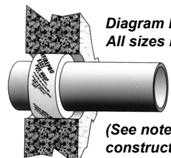
Diagram C - WALL SEALS B305 32mm, 40mm, 50mm (See note 2, Table 1 for hollow wall construction.)
